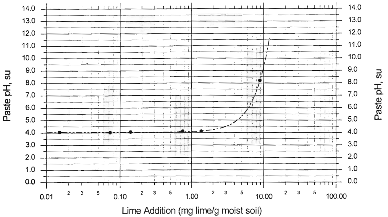
Appendix C Figure 18. Relationship of Paste pH to Quantity of Lime Added to the <1/4" Size Fraction of Sample 12.
