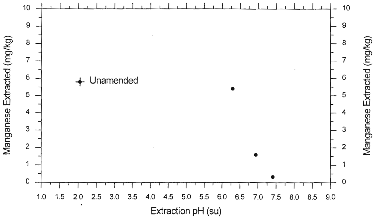
Appendix C Figure 35. Relationship of Extraction pH to Quantity of Manganese Extracted from the <1/4" Size Fraction of Sample 15-1
