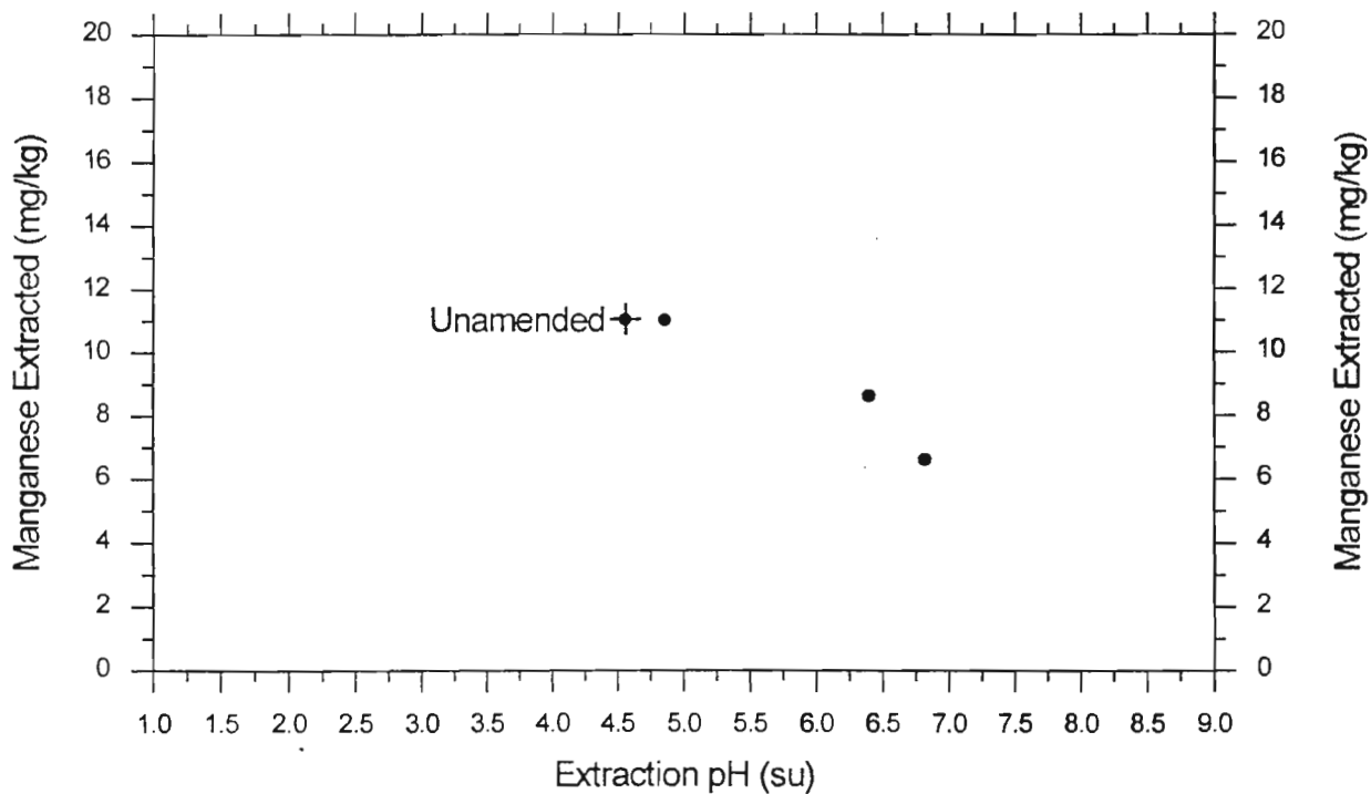
Appendix C Figure 39. Relationship of Extraction pH to Quantity of Managnese Extracted from the <1/4" Size Fraction of Sample 17-3
