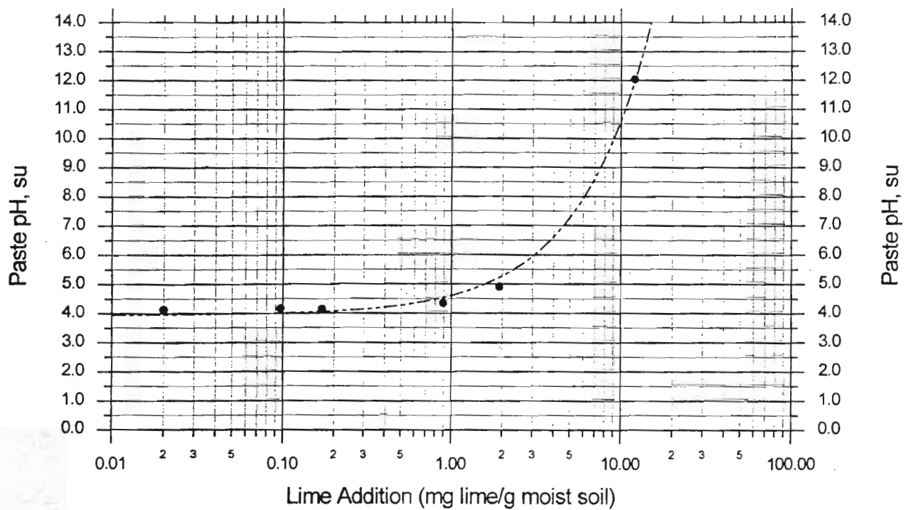
Appendix C Figure 22. Relationship of Paste pH to Quantity of Lime Added to the <1/4" Size Fraction of Sample 14-1
